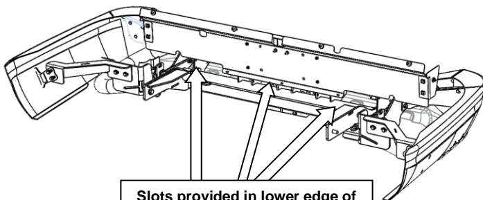
Slots provided in lower edge of beaver panel and RSTB frame brackets
